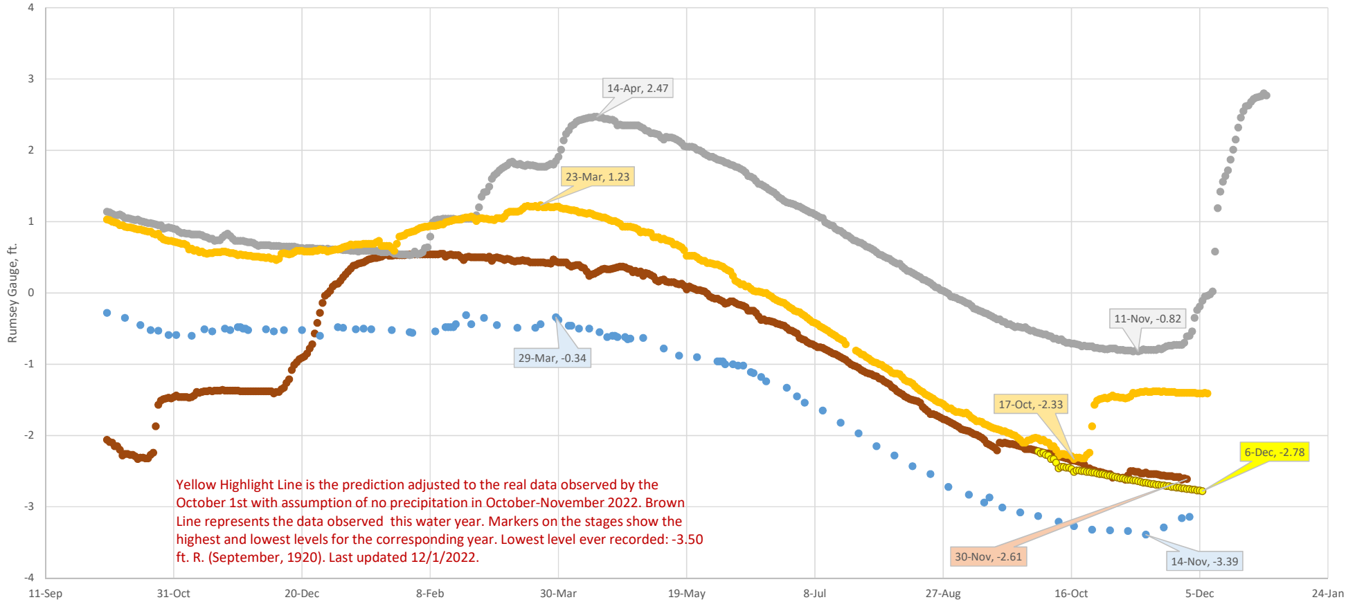
Clear Lake levels: 1977, 2014, 2021, 2022, and 2022 Predicted
